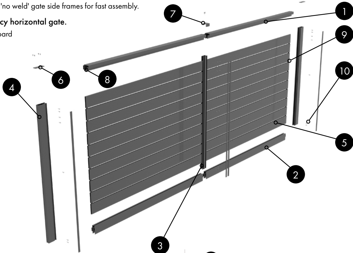
Sliding gate bottom rail 71" or 95" long Order Code: QSSG-1828/2413-BR
